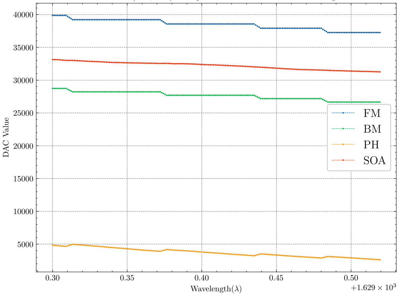
DAC Parameters (400, 450) Interpolated with 3 Intermediate Integer Values
